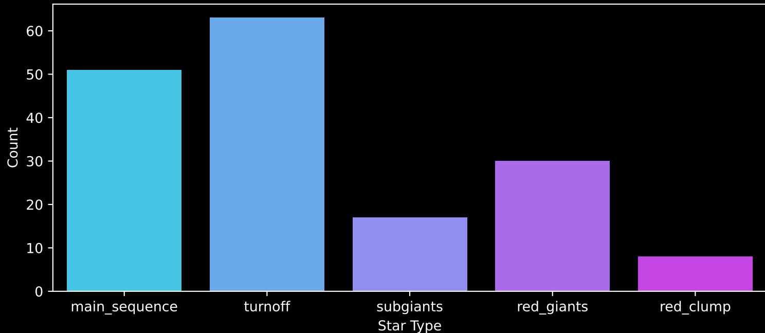
GALAH DR4 Field: [7126] Count plot of Star Type
