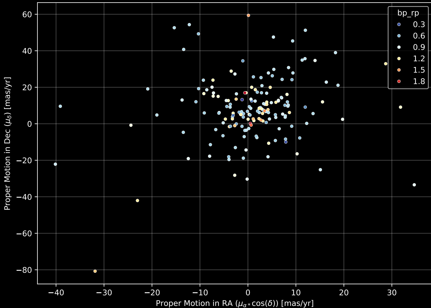
GALAH DR4 Field: [7126] Proper Motion Diagram (n= 169)
