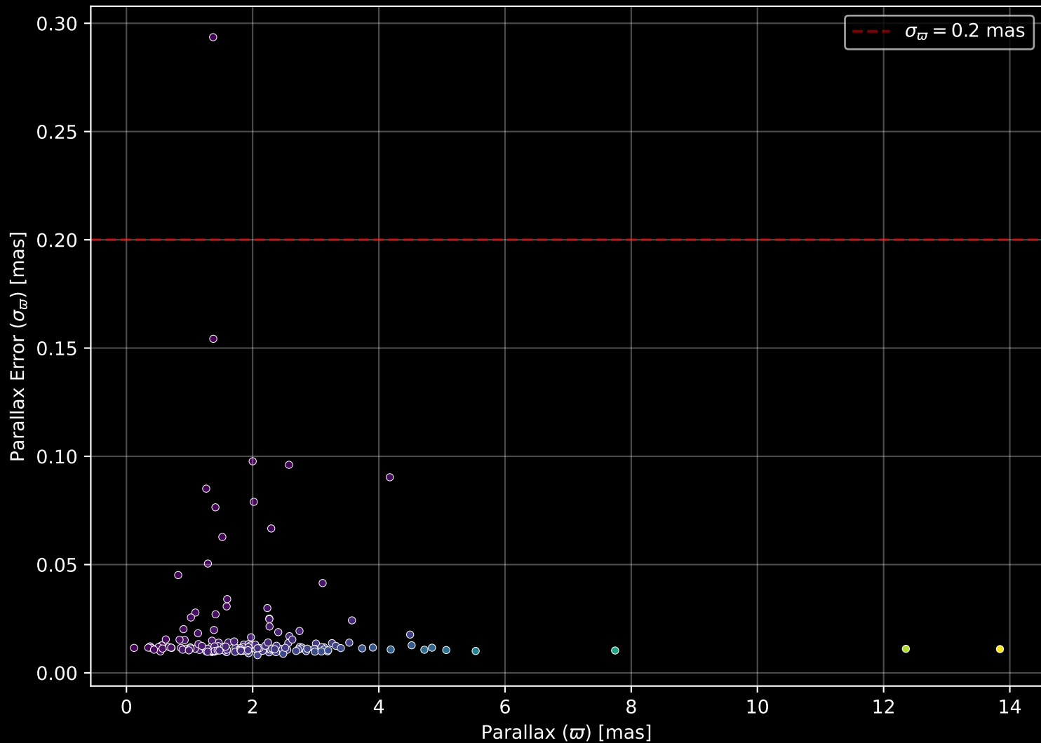
GALAH DR4 Field: [7126] Parallax Quality (n= 169)
