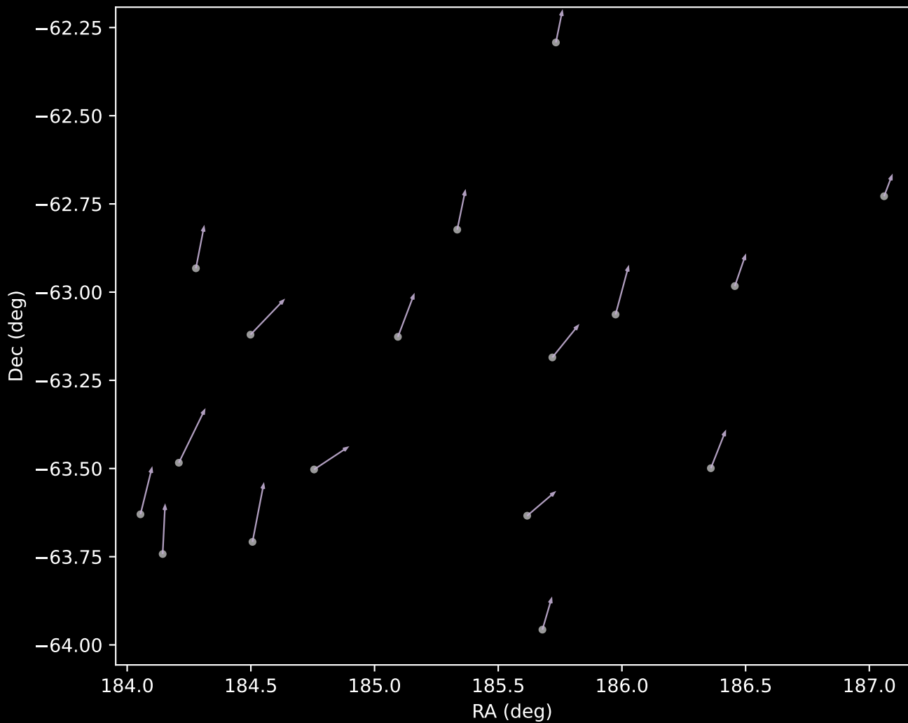
GALAH DR4 Cluster 9 Proper Motion Vectors (n=17)
