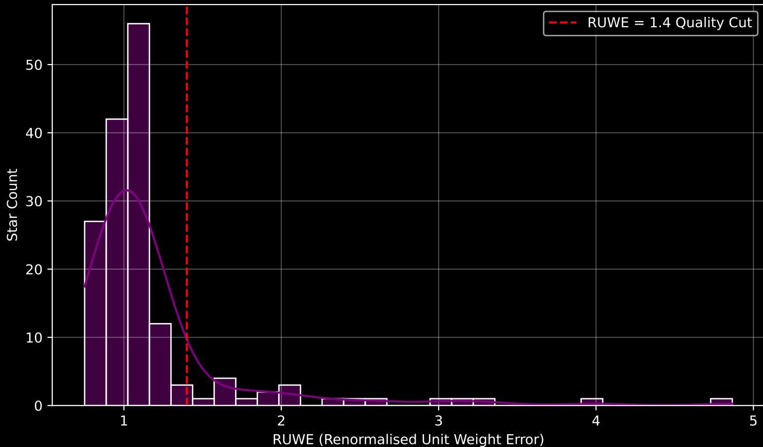
GALAH DR4 Field [7126] RUWE Distribution (n= 159)
